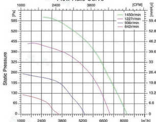
Flow Rate Curve
