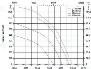
Flow Rate Curve
