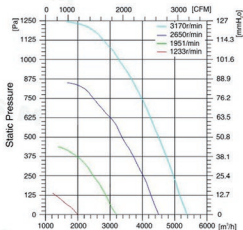
Flow Rate Curve
